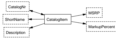
Figure 2.7: C-XML Model Instance for the Catalog of an Acquired Company.
